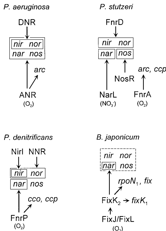
FIG. 30. Positive regulatory circuits controlled by different types of transcription factors in denitrification. Arrows point to boxed groups of target genes or individual operons under the control of a given regulator. The exogenous signals oxygen and nitrate are shown in parentheses where they are correlated with a particular regulator. Structurally and functionally homologous transcription factors are DNR, FnrD, and NNR; structurally but not functionally homologous factors are ANR, FnrA, and FnrP. It is not known whether FixK 2 controls only nar genes or the entire denitrification apparatus in Bradyrhizobium japonicum comparable to the action of ANR. Genetic acronyms: arc , arginine catabolism; cco , cytochrome cbh 3 oxidase; ccp , cytochrome c peroxidase. For a discussion, see the text.
