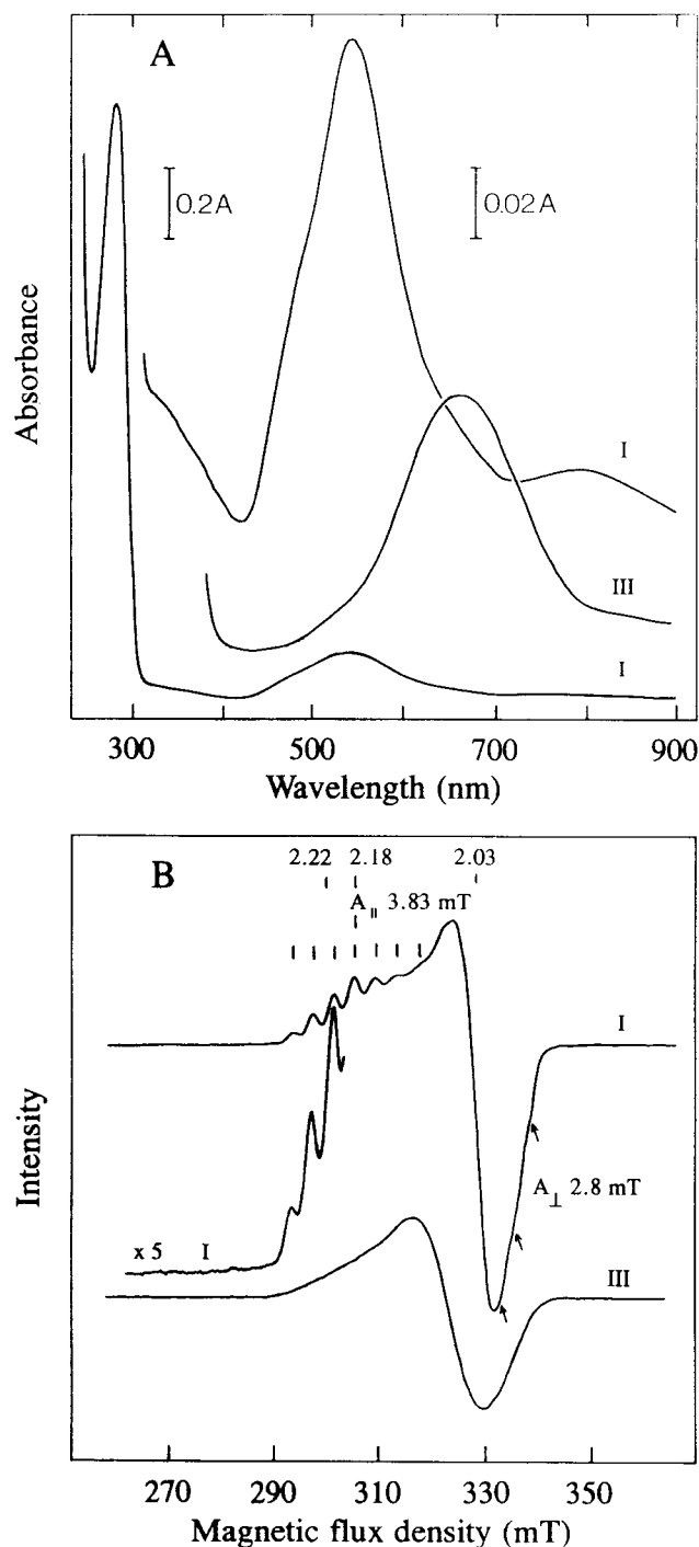
FIG. 20. Electronic absorption (A) and X-band EPR (B) spectra of the two principal forms of N_2O reductase from P. stutzeri ZoBell. I, Resting or purple form; III, blue form obtained by the addition of dithionite to form I. Conditions of recording for EPR spectra: microwave frequency, 9.31 GHz; modulation frequency, 100 kHz; modulation amplitude, 0.5 mT; scan rate, 0.2 mT s^{-1} ; microwave power, 1.6 mW; temperature, 10 K. Reproduced with permission from references 970 and 157.
